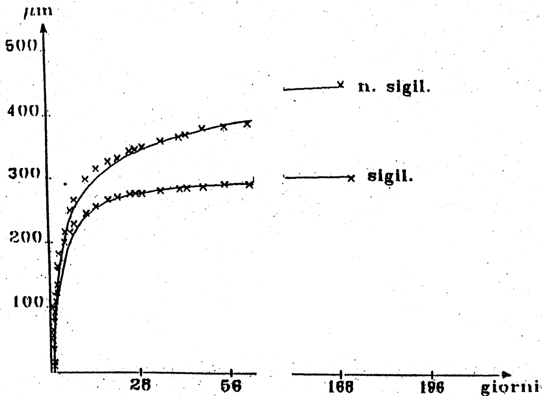
Fig. 9.4 Calcestruzzo f_{c28} 94.5 MPa (cemento 450 Kg/m 3 – microsilice 36 Kg/m 3 – a/c + ms=0,31 – U_R=50\% ) [4.6]
