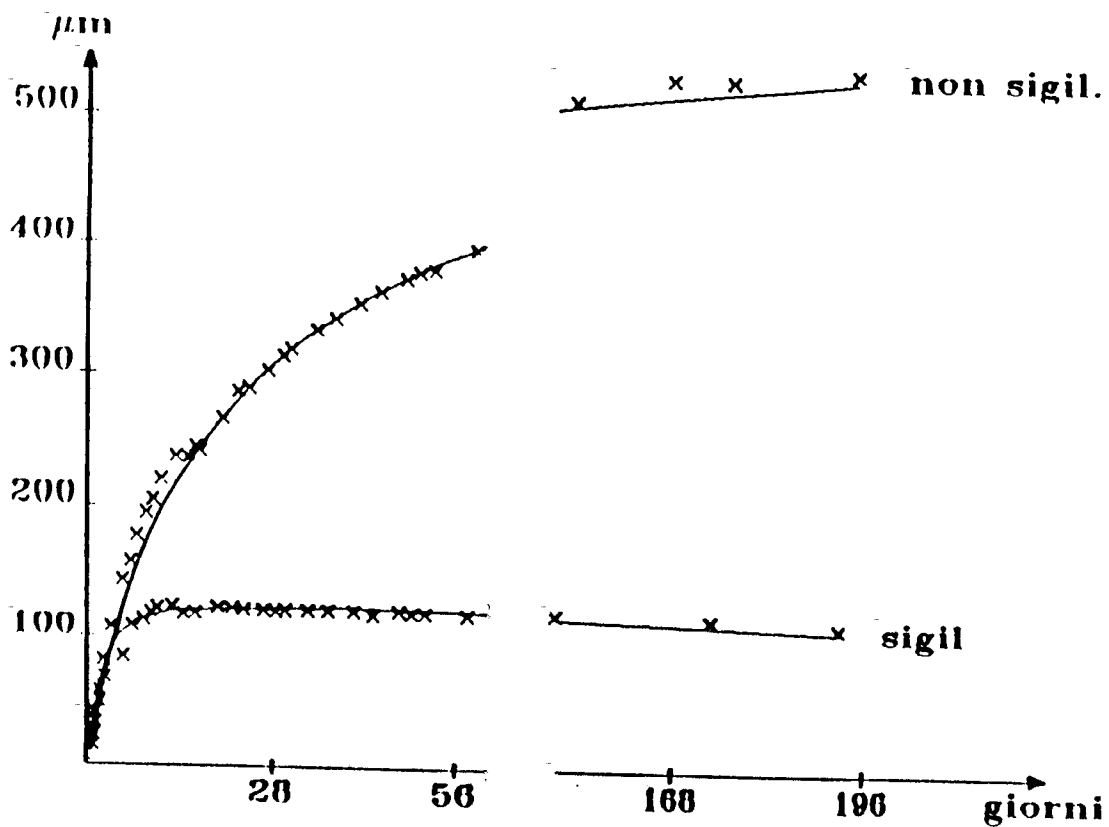
Fig. 8.4 Calcestruzzo f_{c28} 64MPa ( cemento 450 Kg/m 3 – microsilice assente – a/c=0,41 – U_R=50\% )[4.6]
